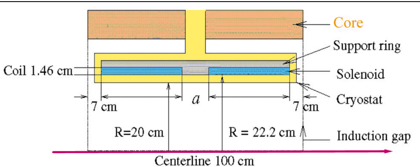
Figure 1: Schematic cross section of an induction linac cell.
