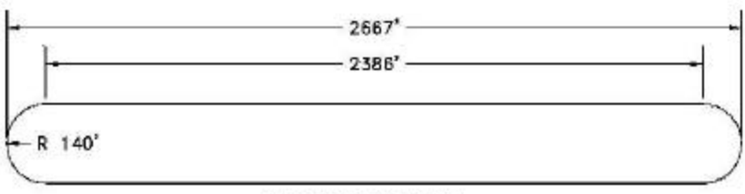
CE 2.1 LATTICE PLAN 1/8"=1'
